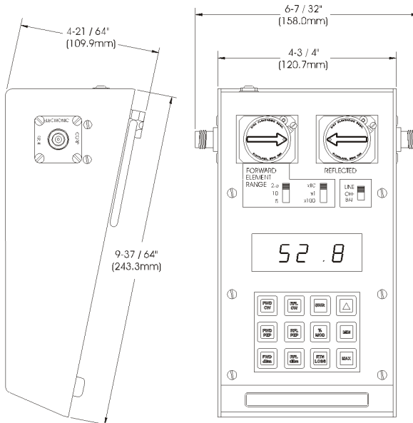
Figure 1 Outline Drawing
