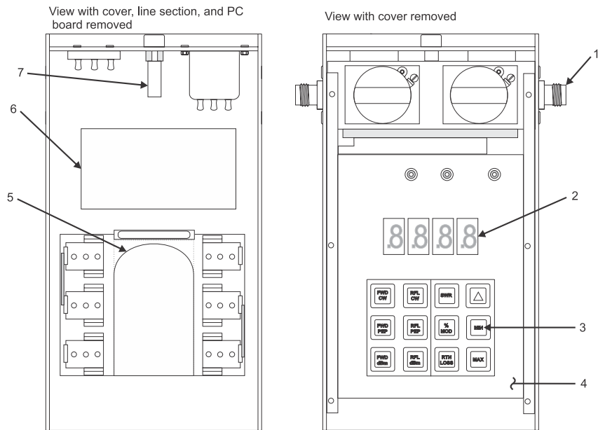
Figure 24 Parts Drawing
