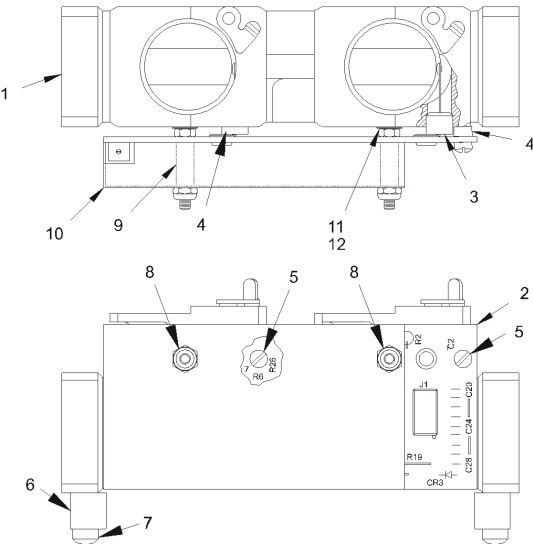
Figure 26 Line Section Assembly (S/N 1724 & above)
