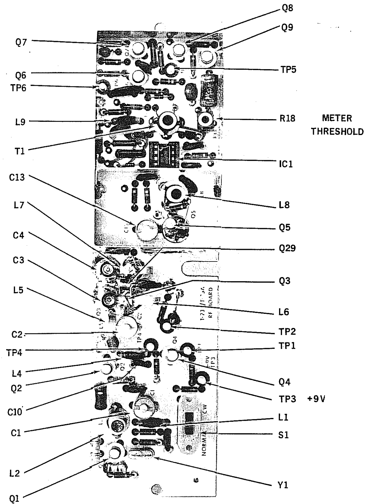
R.F. BOARD
