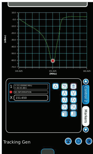
Tracking generator tuning a duplexer
