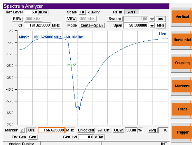
Figure 8. Spectrum Analyzer with Tracking Generator
