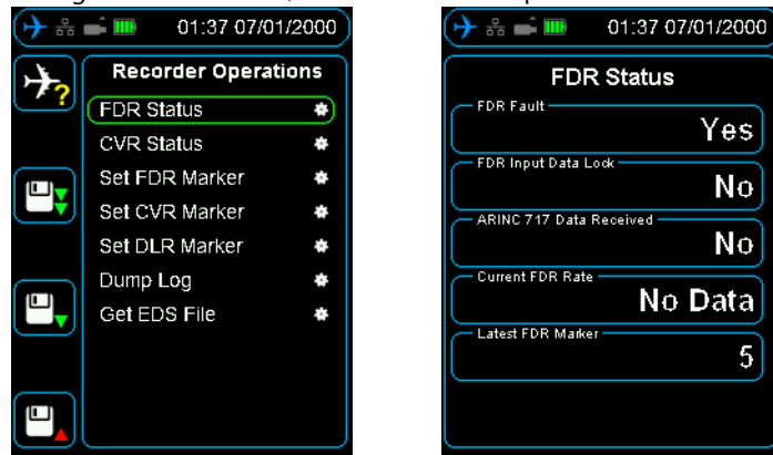
Figure 43.0 FA5000/FA5001 Recorder Operations - FDR Status
