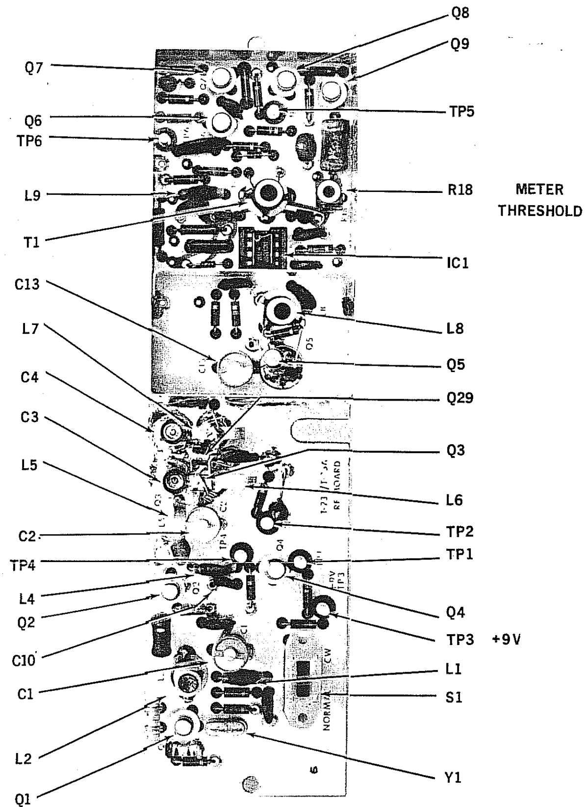
R.F. BOARD
