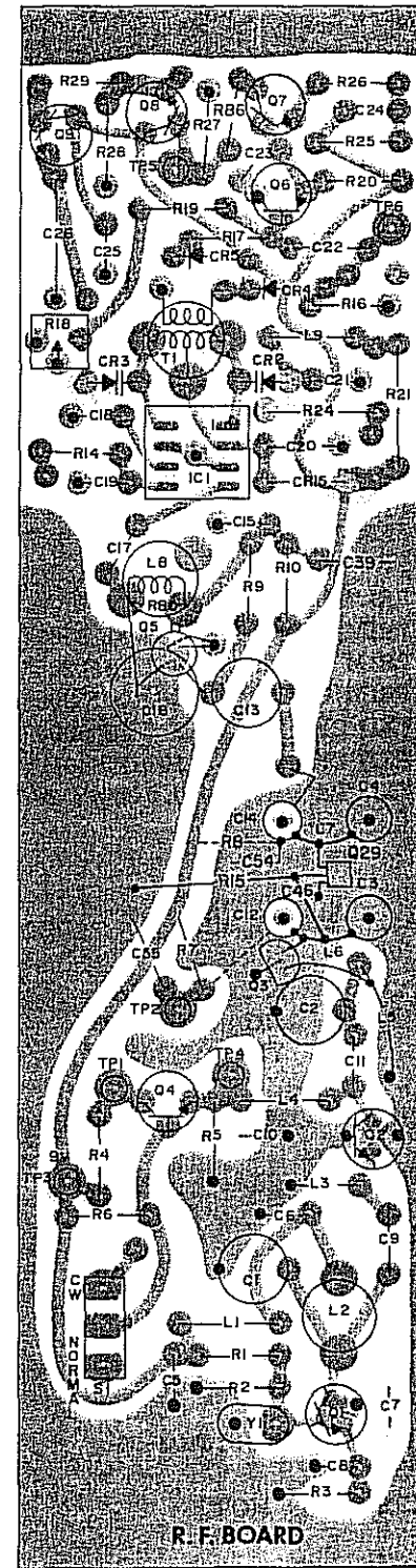
SOLDER SIDE VIEW FIG 4 - 22
