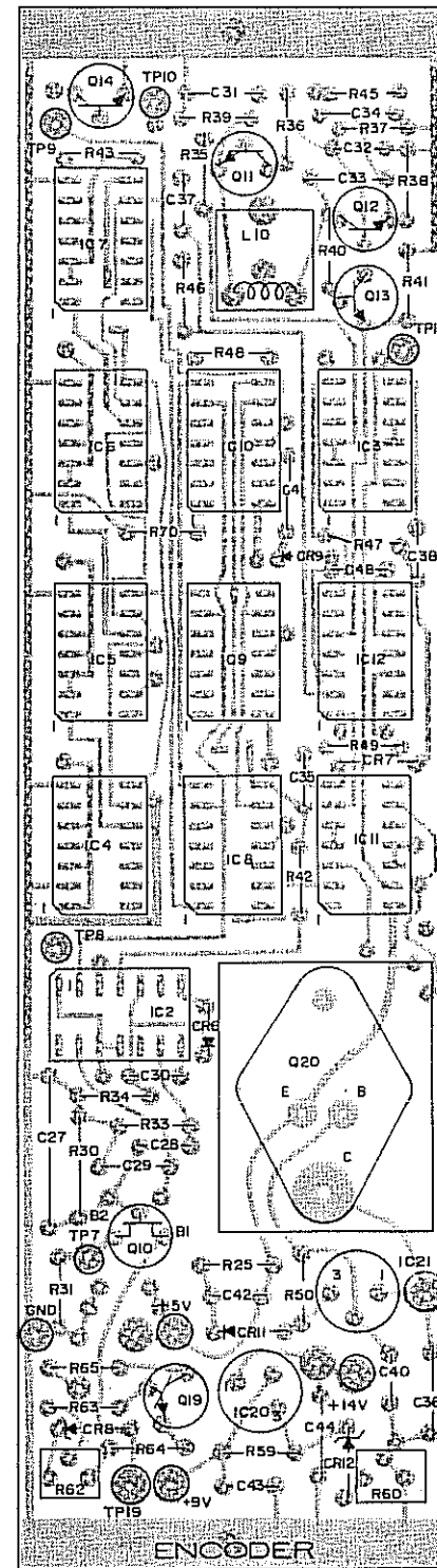
SOLDER SIDE VIEW FIG 4-13
