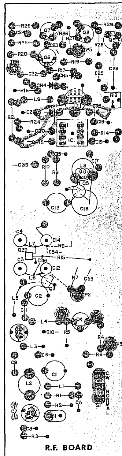
COMPONENT SIDE VIEW FIG 4 - 21
