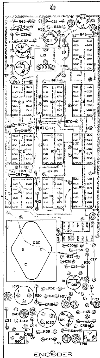
COMPONENT SIDE VIEW FIG 4-12
