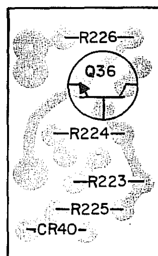
COMPONENT SIDE VIEW
