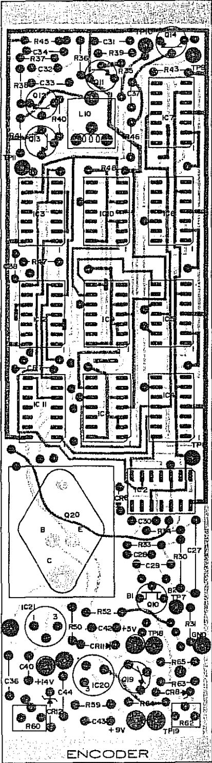
COMPONENT SIDE VIEW fig 4-9
