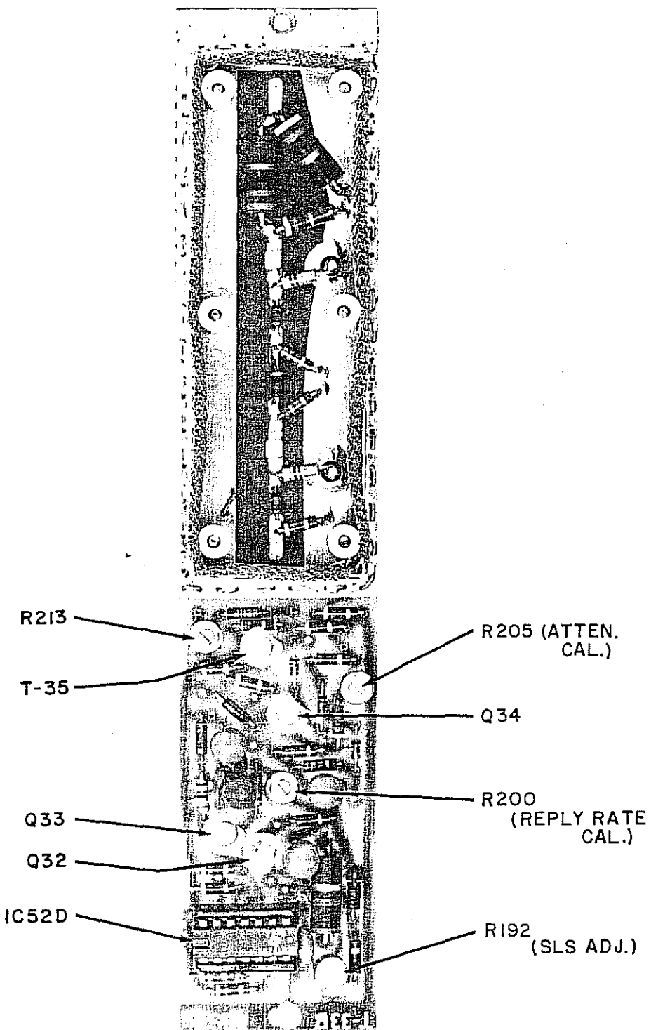
ATTENUATOR BOARD
