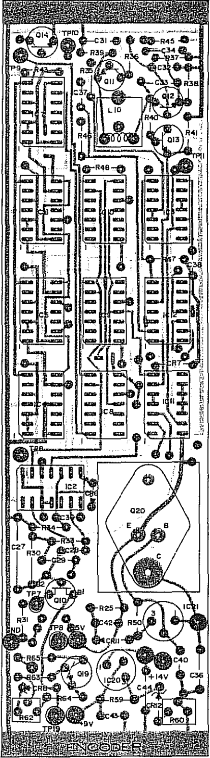
SOLDER SIDE VIEW fig 4-10
