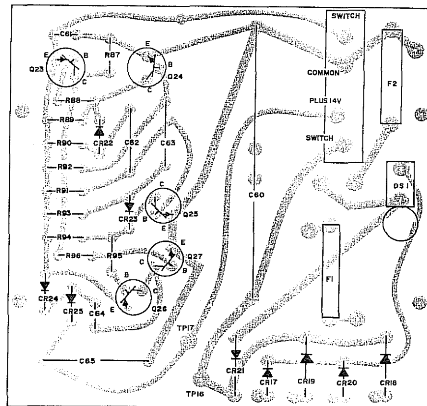
SOLDER SIDE VIEW
