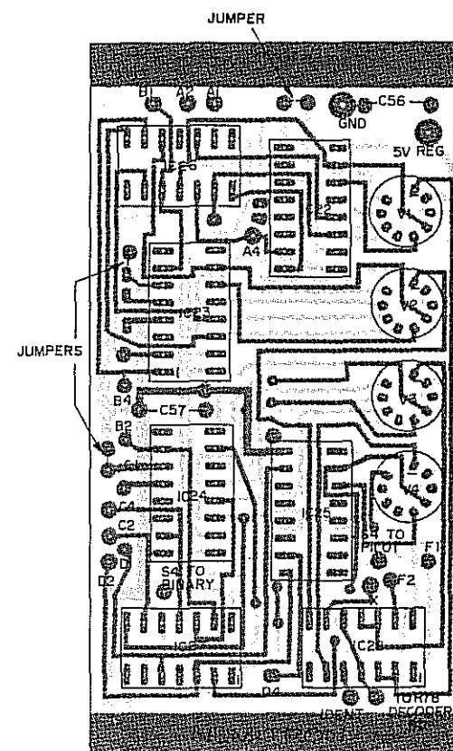
SOLDER SIDE VIEW FIG 4 - 27
