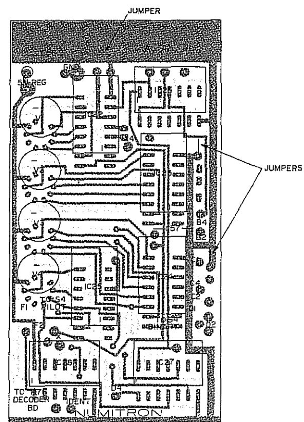
COMPONENT SIDE VIEW FIG 4 - 26
