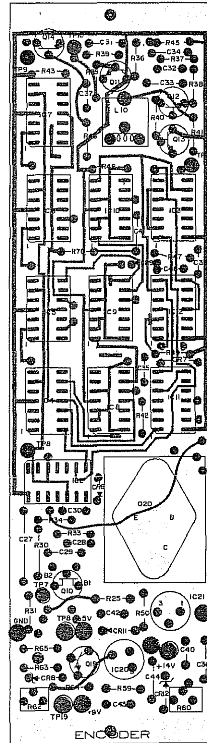
SOLDER SIDE VIEW
