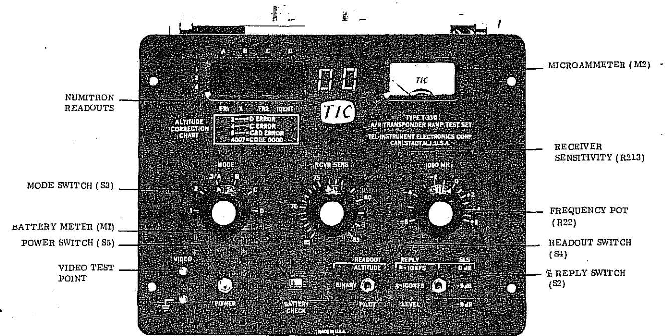
T - 33B FRONT PANEL CONTROL FIG 4 - 3
