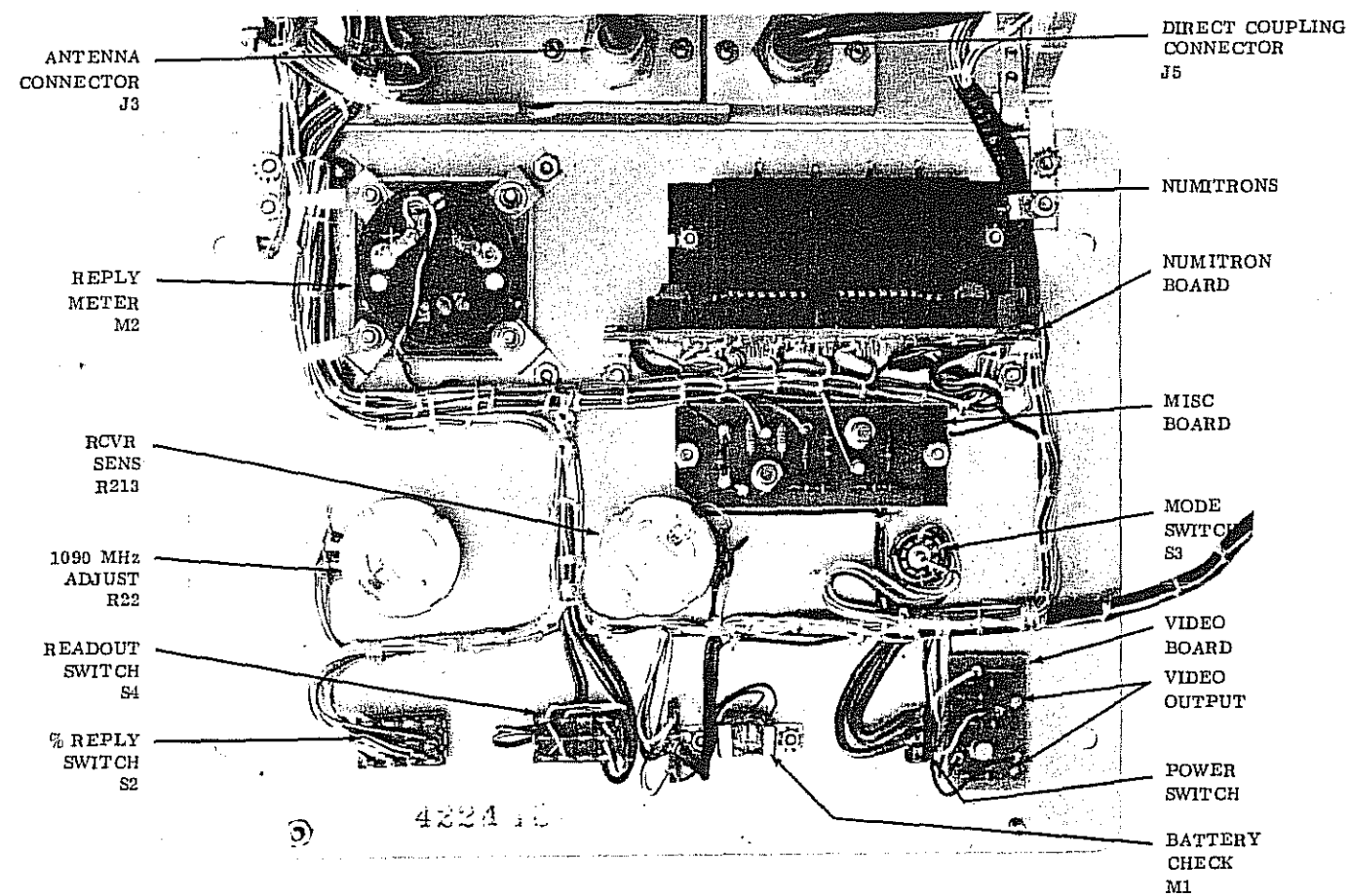
MAIN CHASSIS FIG 4 - 35
