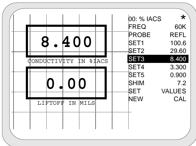
Figure 4-26. Drift Compensation
