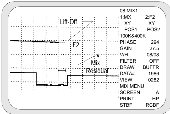
Figure 5-17. Mix Residual
