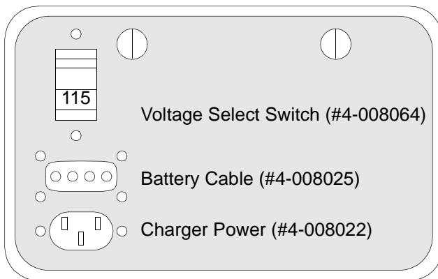
Figure 3-1. Battery Pack Top Assembly Detail
