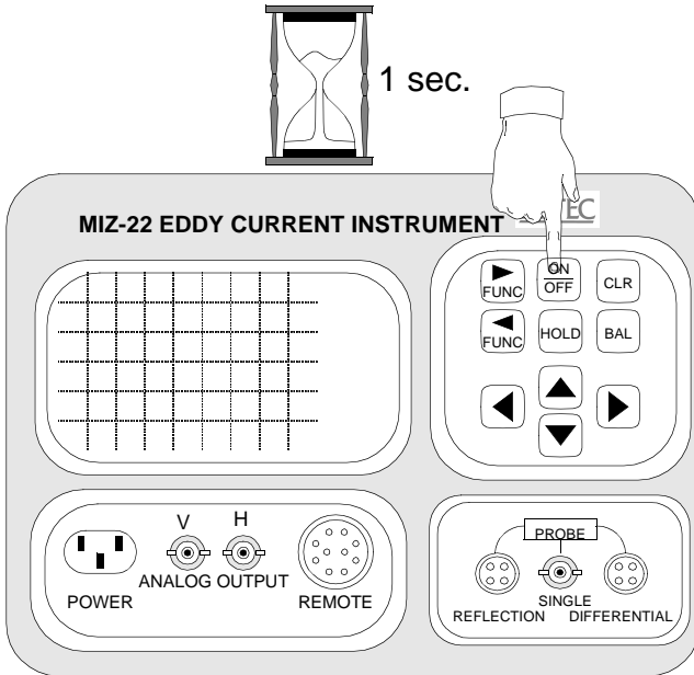
Figure 4-1. ON/OFF Control
