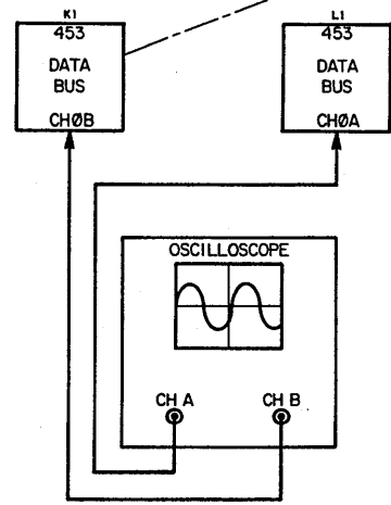
DATA Bus (Channel 1) Evaluation Set-Up Diagram Figure 38
