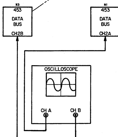
Data Bus (Channel 3) Evaluation Set-Up Diagram Figure 41
