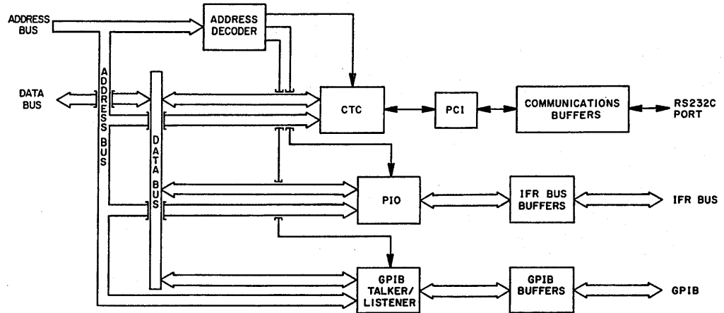
I/O Card Block Diagram Figure 7
