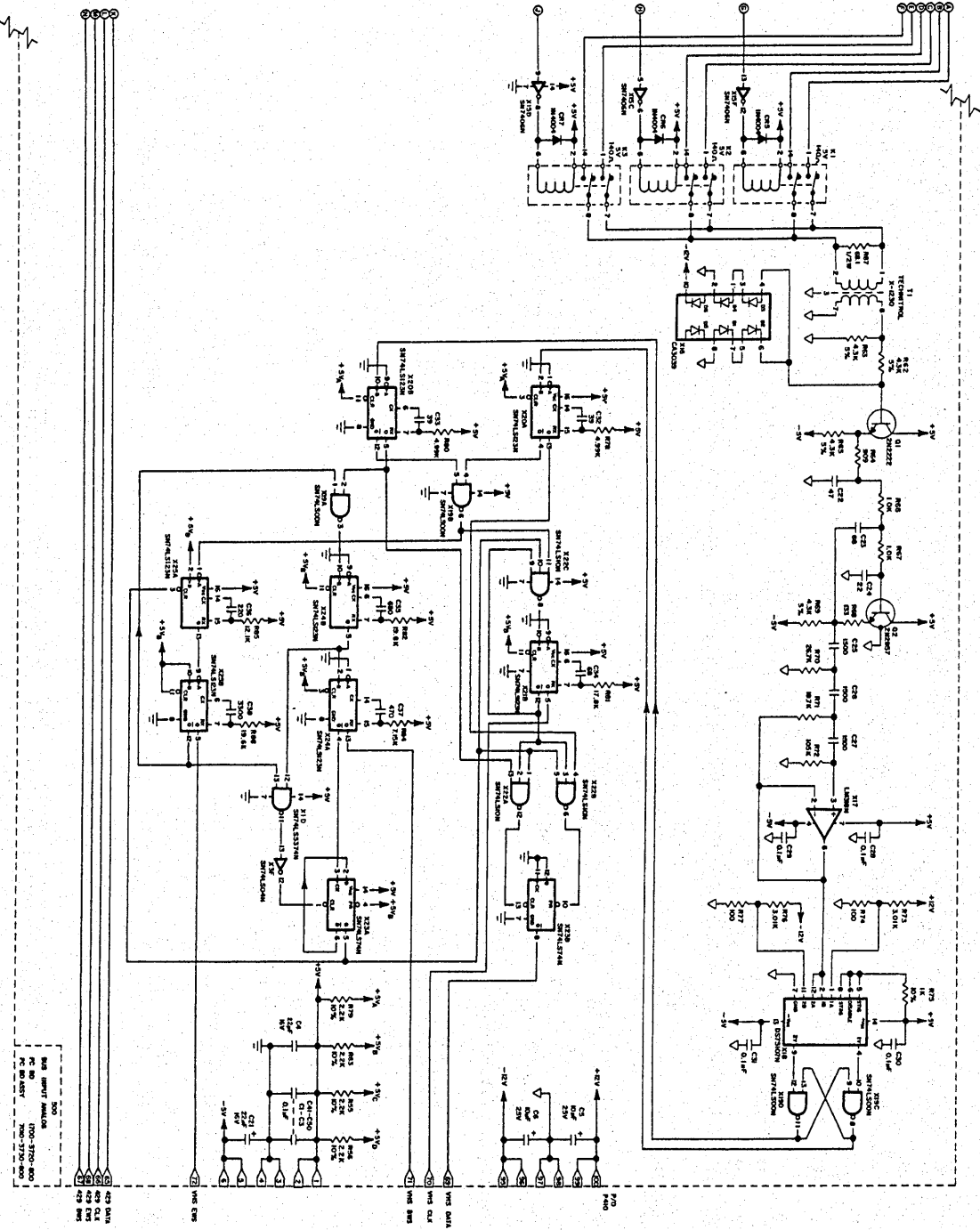
Bus Input Analog Circuit Schematic (Sheet 2 of 2) Figure 92
