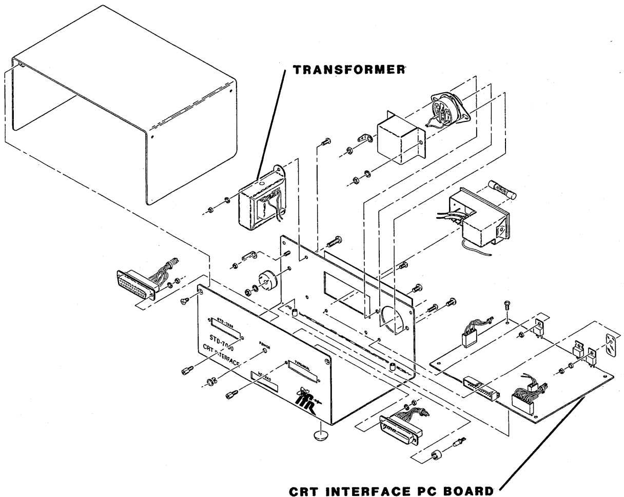
CRT Interface Composite Figure 3
