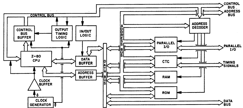
CPU Card Block Diagram Figure 6
