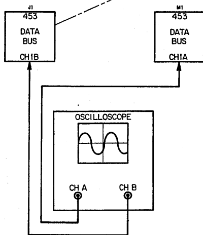
Data Bus (Channel 2) Evaluation Set-Up Diagram Figure 40
