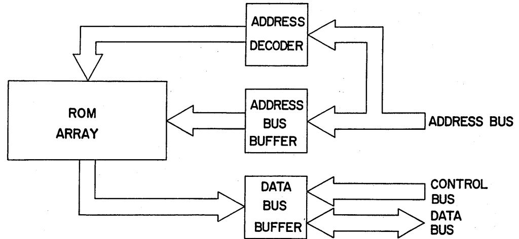
EPROM Card Block Diagram Figure 4
