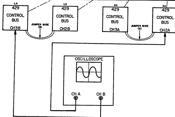
Control Bus (Channels 2 and 3) Evaluation Set-Up Diagram
