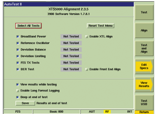
Example of Auto-Test II Display
